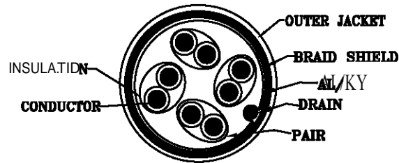
WIRE SECTION
